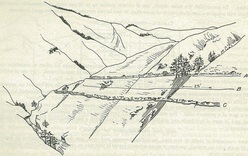
FIG. 2.—A, results on a trail constructed from a well marked grade line; B, grade stakes and a mark 2 to 4 inches wide in the earth on grade between them; C, result on a trail not constructed from a marked grade line. (Par. 42.)
