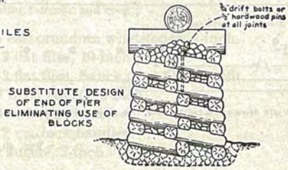
FIG. 39A.—Design of log crib pier, rock filled.
