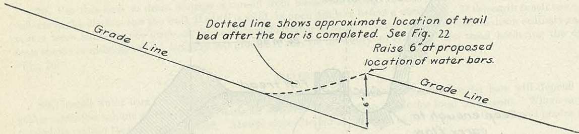
FIG. 21.—Showing profile of grade line at proposed location of water bars. (Par. 81.)
