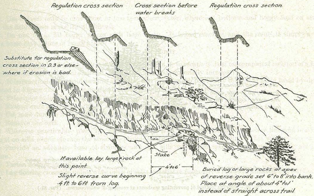
FIG. 22.—Lateral section of trail showing water-break log. (Par. 81.)
