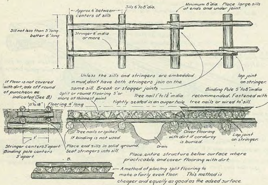
FIG. 26.—Showing end and side views of ordinary sill and stringer corduroy with puncheon or pole flooring.
