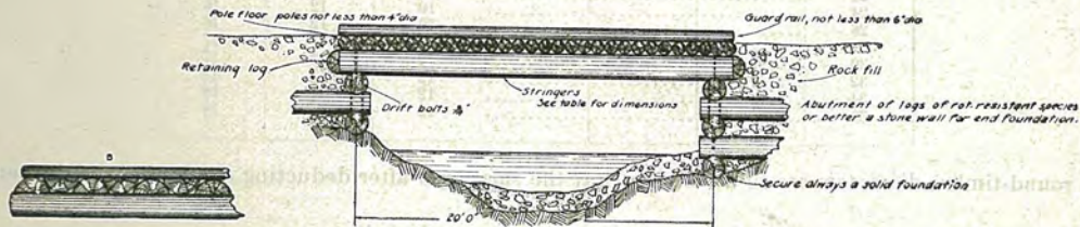
Elevation. Fig. 36
