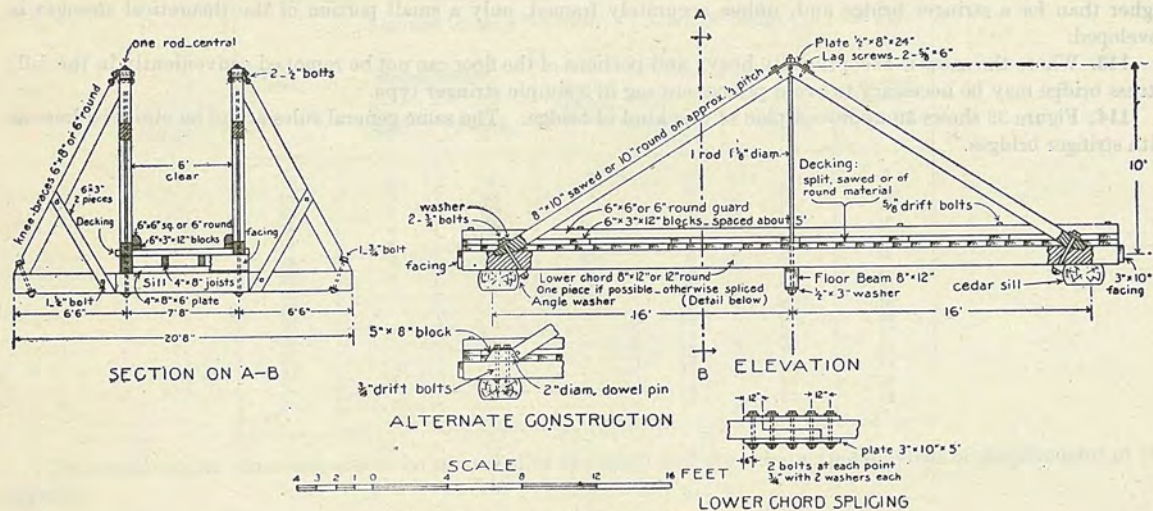
FIG. 39.—Plan of King truss bridge.
