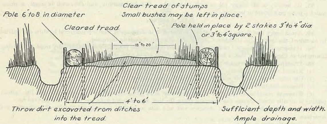
FIG. 24.—Showing cross section of trail on flat soft wet ground where ditch on each side will provide a dry and more durable tread than corduroy: (Par. 85.)
